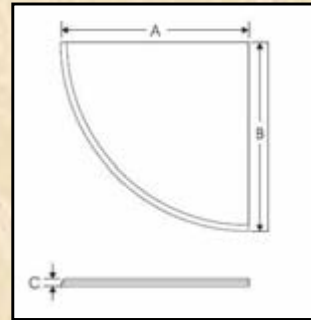
1" Hearth Tile Radius Corner
